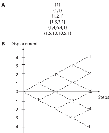
Fig. 2. Random walks results in a binomial distribution. (A) Example of the binomial distribution produced by five steps. (B) Possible routes for an unbiased random walk starting at the origin (0). Numbers represent the number of possible walks to reach a specific distance from the origin.
