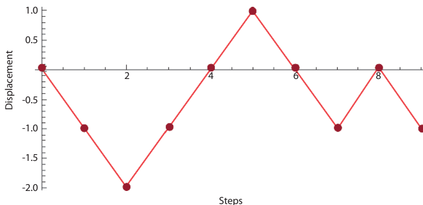
Fig. 1. Plot of a random walk.
