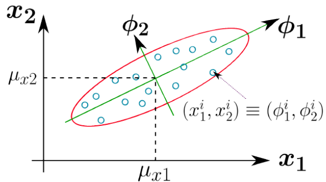
Figure 3: The PCA Transformation
